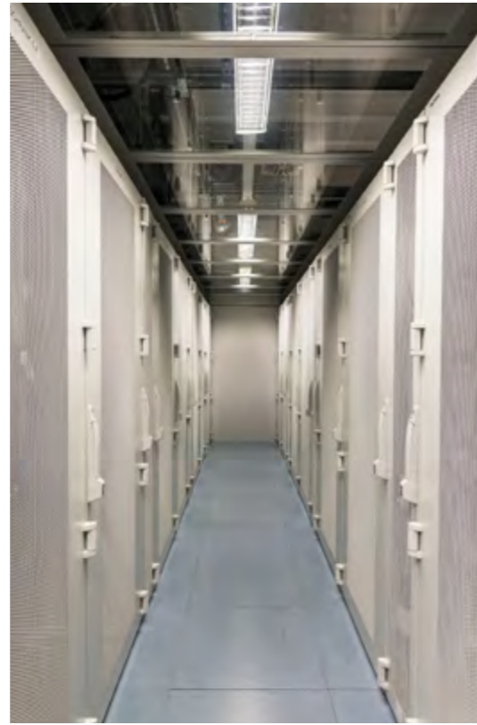
dtm cold aisle containment system combined with third-party racks
