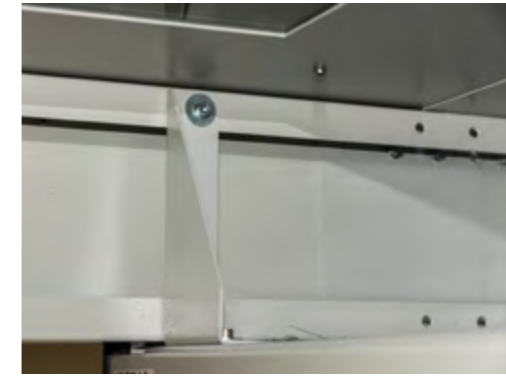
dtm cold aisle containment system combined with third-party racks
